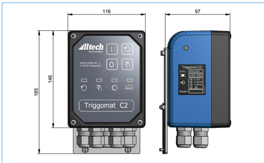
Dimensional drawing TRIGGOMAT
